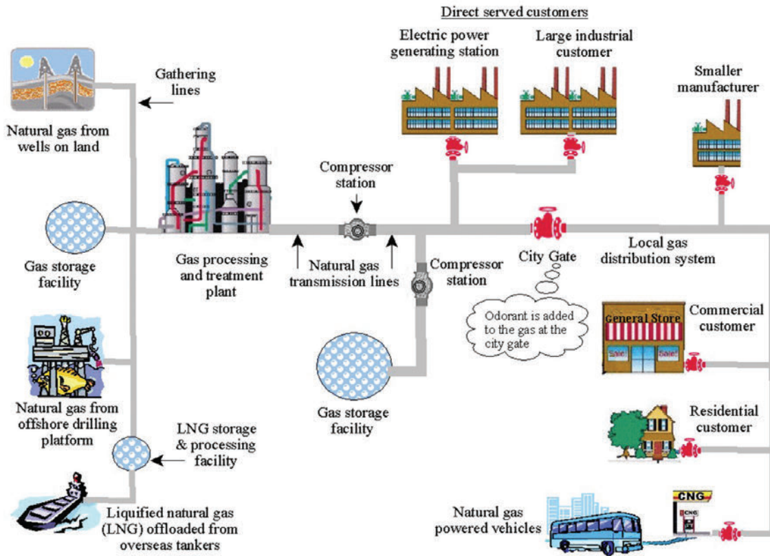
Natural gas pipeline system from production to end user. (Source: U.S. DOT PHMSA)
